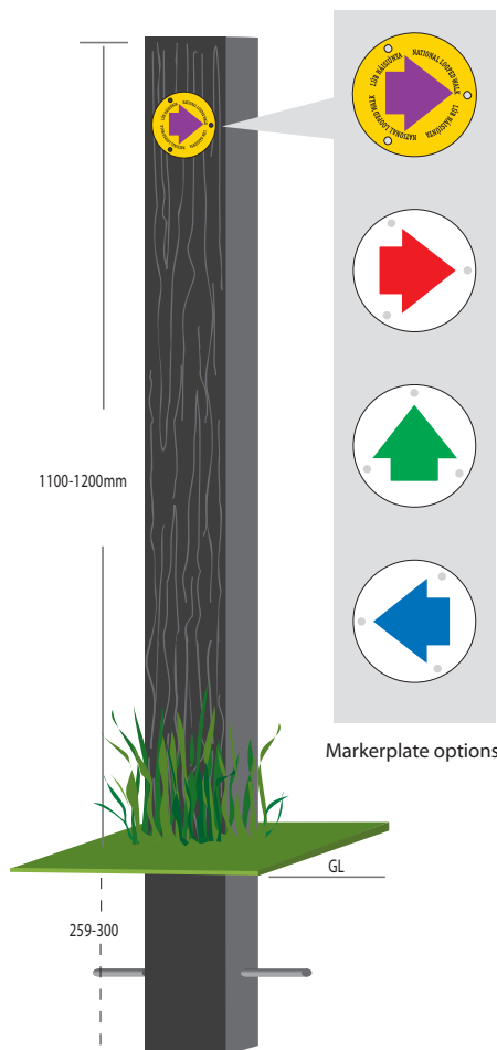
National Looped Walk Markerpost
