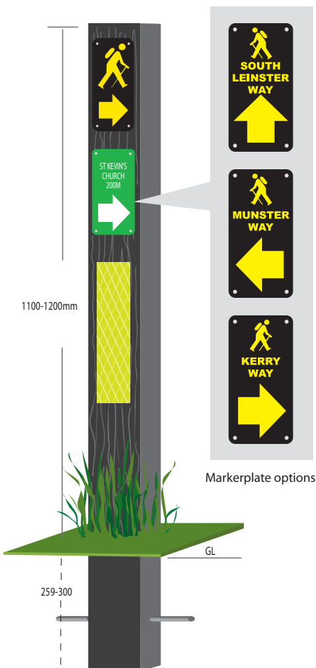
National Waymarked Ways Markerpost
