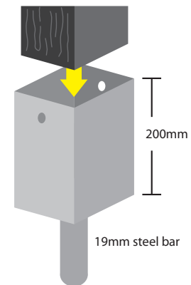
Markerpost Sleeve for Mountainous Regions
